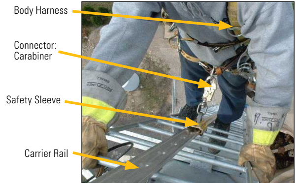
Figure 1: Components (parts) of a ladder safety device [fall protection equipment]. (Illustrates correct navel D-ring to safety sleeve connection for this specific device.)
