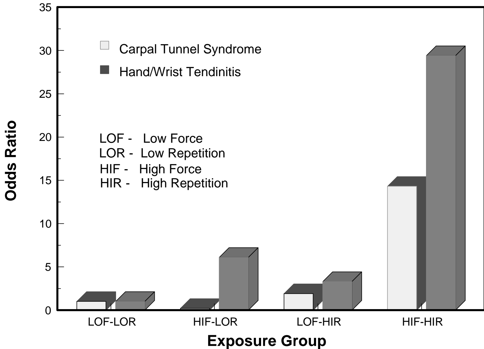
Figure V-6 Relationship Between Exposure to Risk Factors and Risk of Upper Body Musculoskeletal Disorders
