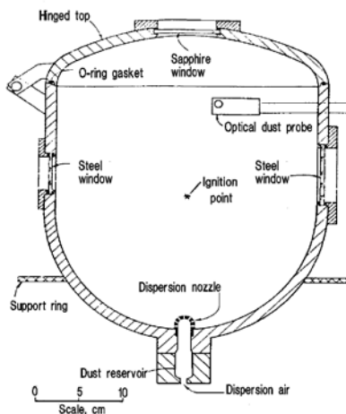
Figure 1: 20-Liter Explosibility Test Chamber
